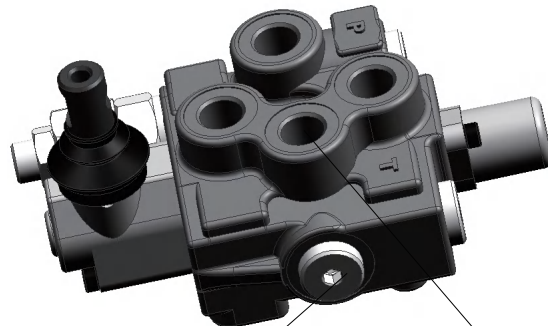
Front port plugged T port on the top
