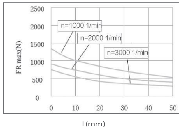
FO=600 N
