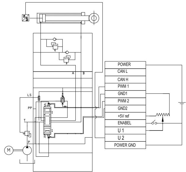
Speed control 2
