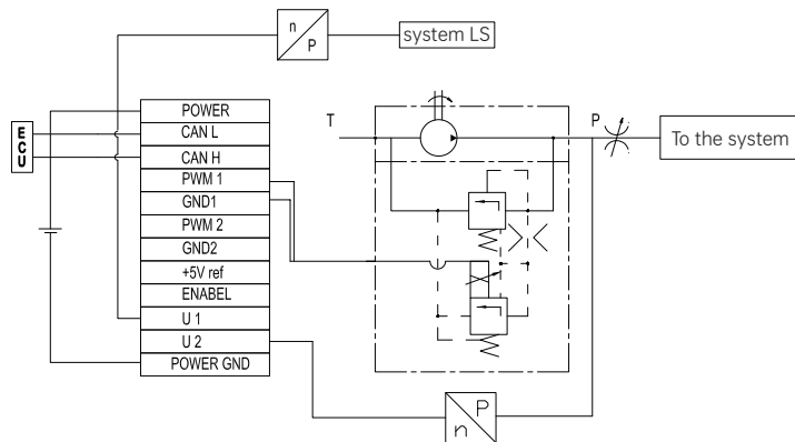
Load-sensitive gear pump
