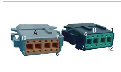
Sheath Connector DTM06-12SA Gray DTM06-12SB Black
