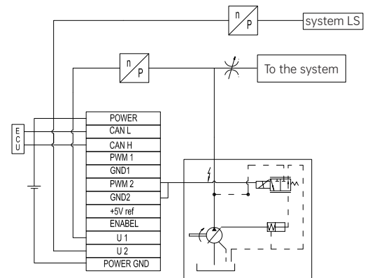
Load-sensitive variable displacement pump
