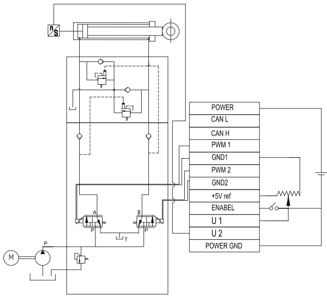
Speed control 1
