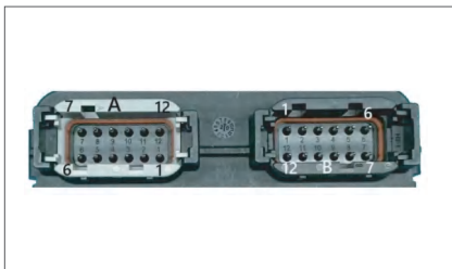
Controller connector DTM13-12PA-12PB-R008
